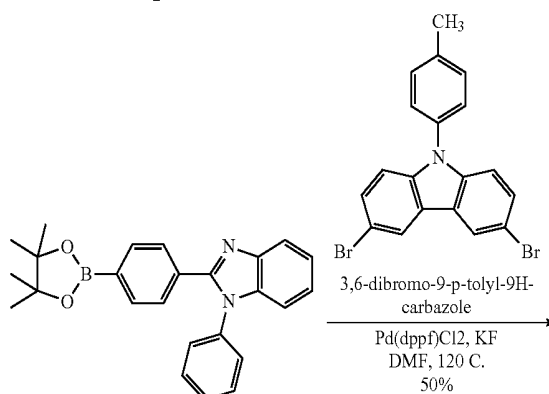
1-phenyl-2-(4-(4,4,5,5-tetramethyl-1,3,2-dioxaborolan-2-yl)phenyl)-1H-benzo[d]imidazole
