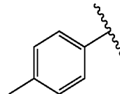
4-methylphenyl
