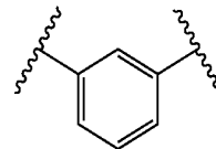
m-phenylene
