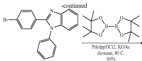
2-(4-bromophenyl)-1-phenyl-1H-benzo[d]imidazole
