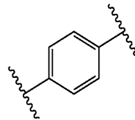
p-phenylene
