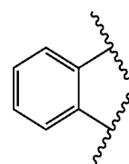
o-phenylene
